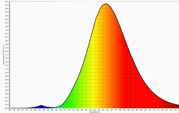
PowerSpectrum @ 1 meter Source Sensor Distance
